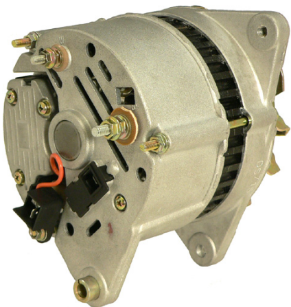
ALU0007 IR/EF; 12-VOLT; 70 AMP; LESTER 12091; PIC 280-339; USED ON FORD AGRICULTURAL AND INDUSTRIAL, MASSEY FERGUSON REPL.: 24274, 54022337, -2528, 63324274
